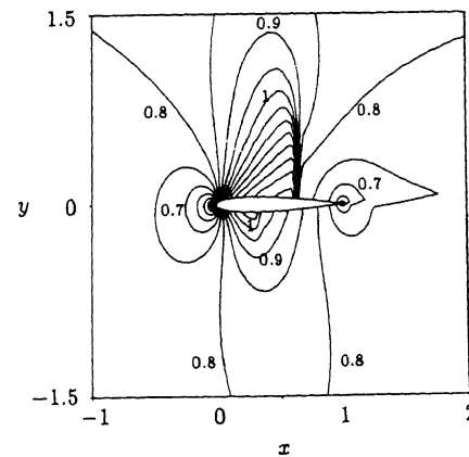
Figure 7: Iso-line plots of the Mach number for the transonic flow around a NACA0012 airfoil; \alpha = 1.25^\circ ; M_\infty = 0.8 ; locally refined grid: L = 5 ; uniform grid: L = 4 .
